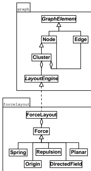
Figure 3: A Class diagram showing the essential classes implementing Wilma’s graph and force model engines.
